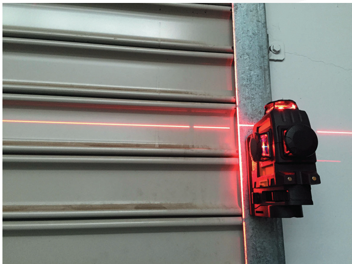
Unit pictured above is the 3L360R three line laser level. Housing and magnetic bracket is the same as supplied with the 2L360 models
